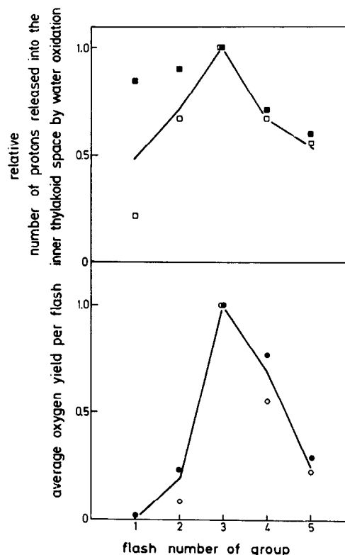
Fig.2. Oscillatory pattern of oxygen evolution and proton release due to system II electron transport with water as electron donor in a flash train of single turnover flashes. The curves give the theoretical values obtained for the present model with the additional assumption of a dark oxidation degree of M to be 0.65 and average probabilities of missings and double hits of 0.1 and 0.05, respectively. The experimental data indicated by squares and circles are redrawn from ref. [3,10] (open circles), ref. [16] (open squares) and ref. [17] (closed symbols). The activity in the third flash is used for normalization.
